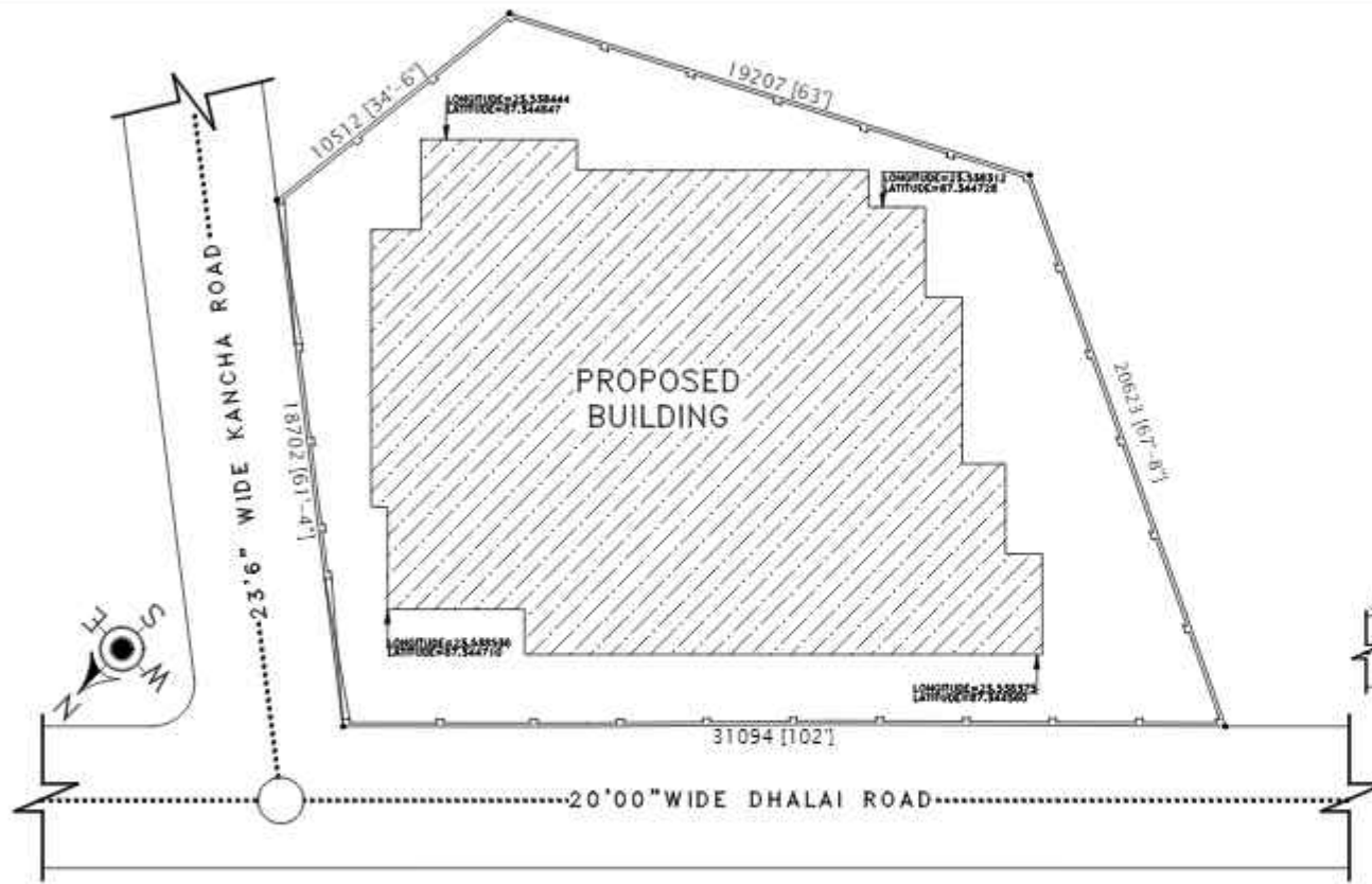
(A) SITE PLAN SCALE 1:100
